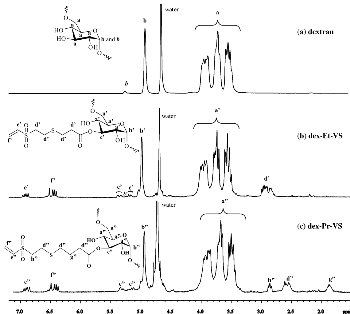
Figure 1. ^1\text{H} NMR spectra ( \text{D}_2\text{O} ) of (a) dextran, (b) dex-Et-VS (Table 1, entry 3), and (c) dex-Pr-VS (Table 1, entry 10). The substitution at position C-3 is given as an example.
