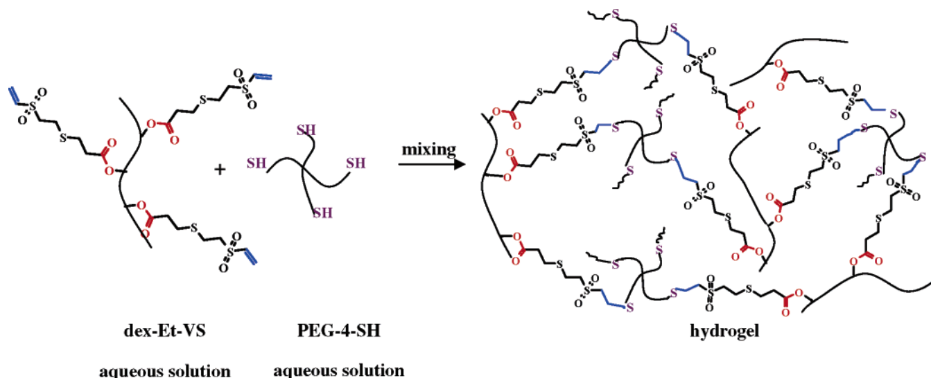
Figure 2. Schematic representation of the Michael type addition between dex-VS and PEG-SH, shown for dex-Et-VS and PEG-4-SH.
