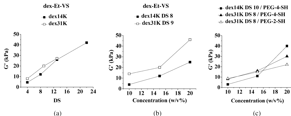
Figure 5. Storage modulus plateau values of dex-Et-VS and dex-Pr-VS hydrogels in HEPES buffered saline at pH 7 and 37 °C: (a) dex14K-Et-VS and dex31K-Et-VS with PEG-4-SH as a function of the degree of substitution (DS); (b) dex14K-Et-VS and dex31K-Et-VS with PEG-4-SH as a function of the concentration; (c) dex14K-Pr-VS DS 10 with PEG-4-SH and dex31K-Pr-VS DS 8 with PEG-4-SH or PEG-2-SH as a function of the concentration.
