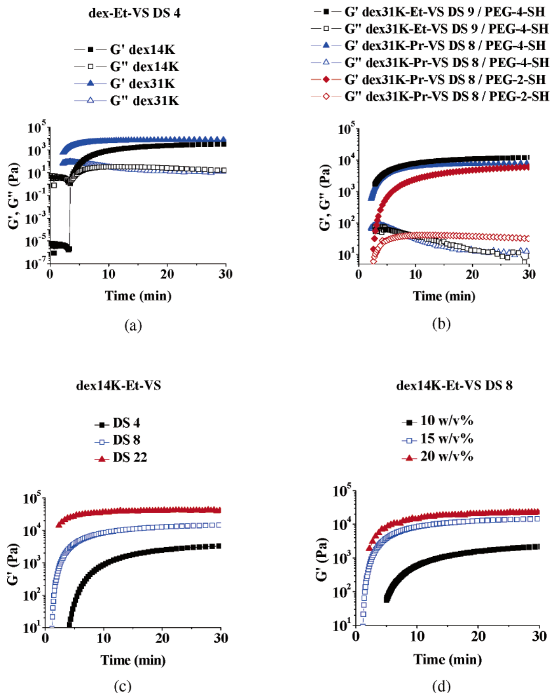
Figure 4. Storage modulus ( G' ) and the loss modulus ( G'' ) as a function of time of dex-VS/PEG-SH mixtures in HEPES buffered saline at pH 7 and 37 °C: (a) dex14K-Et-VS DS 4 and dex31K-Et-VS DS 4 with PEG-4-SH at 15% w/v concentration; (b) dex31K-Et-VS DS 9 with PEG-4-SH and dex31K-Pr-VS DS 8 with PEG-4-SH or PEG-2-SH at 10% w/v concentration; (c) dex14K-Et-VS at DS 4, 8, and 22 at 15% w/v concentration; (d) dex14K-Et-VS DS 8 at 10, 15, and 20% w/v concentration.
