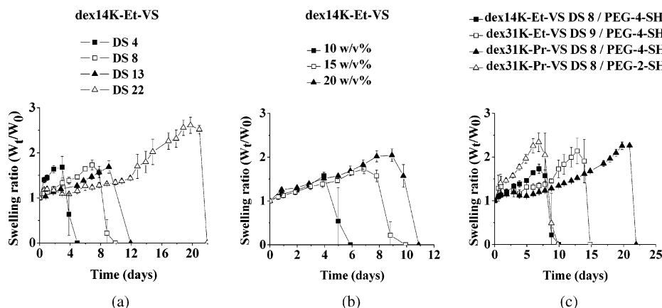
Figure 6. Swelling ratio ( W_t/W_0 ) profiles of dex-VS hydrogels in HEPES buffered saline at pH 7 and 37 °C ( n = 3 ): (a) dex14K-Et-VS with PEG-4-SH at DS 4, 8, 13, and 22 at 15% w/v concentration; (b) dex14K-Et-VS DS 8 with PEG-4-SH at concentrations of 10, 15, and 20% w/v; (c) dex14K-Et-VS DS 8 and dex31K-Et-VS DS 9 with PEG-4-SH and dex31K-Pr-VS DS 8 with PEG-4-SH or PEG-2-SH at 15% w/v concentration.
