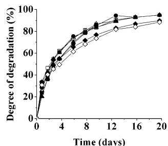
Figure 8. Degree of degradation of dex-VS conjugates in PBS at pH 7 and 37 °C as determined by ^1\text{H} NMR: dex14K-Et-VS DS 4 (■), DS 8 (□), DS 13 (▲), and DS 22 (△); dex31K-Et-VS DS 13 (●), dex14K-Pr-VS DS 10 (◆), and dex31K-Pr-VS DS 8 (◇).
