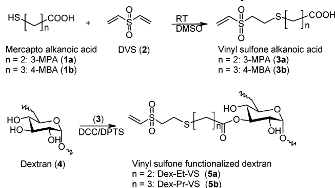
Scheme 2. Schematic Representation of the One-Pot Synthesis Procedure of Dextran Vinyl Sulfone Conjugates with an Ethyl Spacer (Dex-Et-VS) or a Propyl Spacer (Dex-Pr-VS) between the Thioether and Ester Groups
