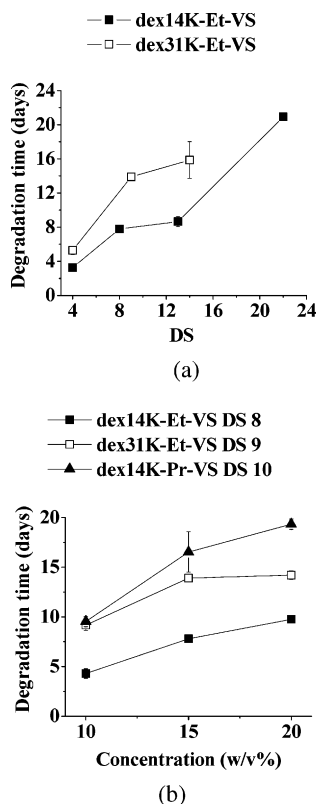
Figure 7. Plots of degradation times vs DS or concentration of dex-Et-VS hydrogels cross-linked with PEG-4-SH in HEPES buffered saline at pH 7 and 37 °C ( n = 3 ): (a) dex14K-Et-VS and dex31K-Et-VS as a function of the DS at 15% w/v concentration; (b) dex14K-Et-VS DS 8, dex31K-Et-VS DS 9, and dex14K-Pr-VS DS 10 as a function of the concentration.
